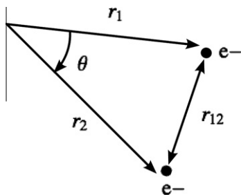
Figure 1. The basic coordinates of a two-electron system.
