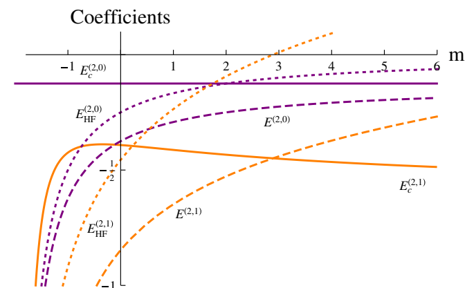
Figure 2. Coefficients of the exact (dashed), HF (dotted) and correlation (solid) energies with respect to m , for v(r) = 1 (Eqs. (75)–(77)).
