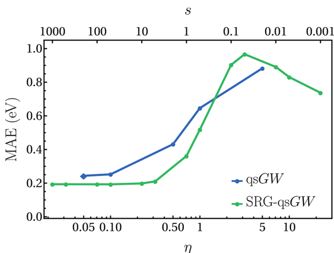
Figure 6. Evolution of the SRG-qsGW (green) and qsGW (blue) MAEs for the principal IPs of the GW 50 test set as functions of s and \eta , respectively. The bottom and top axes are related by s = 1/(2\eta^2) . A different marker has been used for qsGW at \eta = 0.05 because the MAE includes only 48 molecules.
